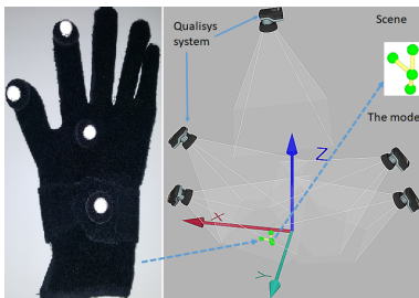
Fig. 2. Left picture shows the black glove that contains 4 infrared reflective markers, the right picture summarizes the whole scene with the emplacement of the motion capture cameras, and the model in green color.
