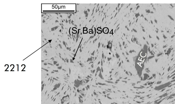
Figure 2. SEM (backscattered electron, BSE) image of a polished cross-section in the central part of the tube showing major second phases (\text{Ba}_{0.13}\text{Sr}_{0.87})\text{SO}_4 and (\text{Sr}_{0.6}\text{Ca}_{0.4})\text{CuO}_2 (1:1AEC) in the Bi-2212 matrix.
