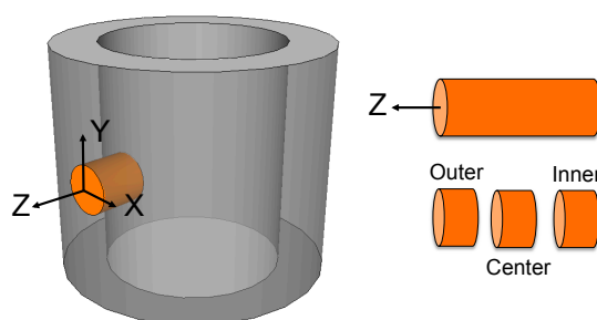
Figure 1. Reference frame of the Bi-2212 tube and sample cutting procedure.
