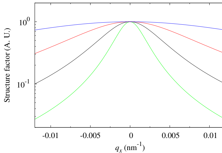
Figure 2. Structure factors proportional to the Lorentzian function, 1/\{1 + (q_x \cdot \xi_{\parallel})^2\} . Green, black, red, and blue line indicates the profile with \xi_{\parallel} = 500, 250, 125, and 50 nm, respectively.
