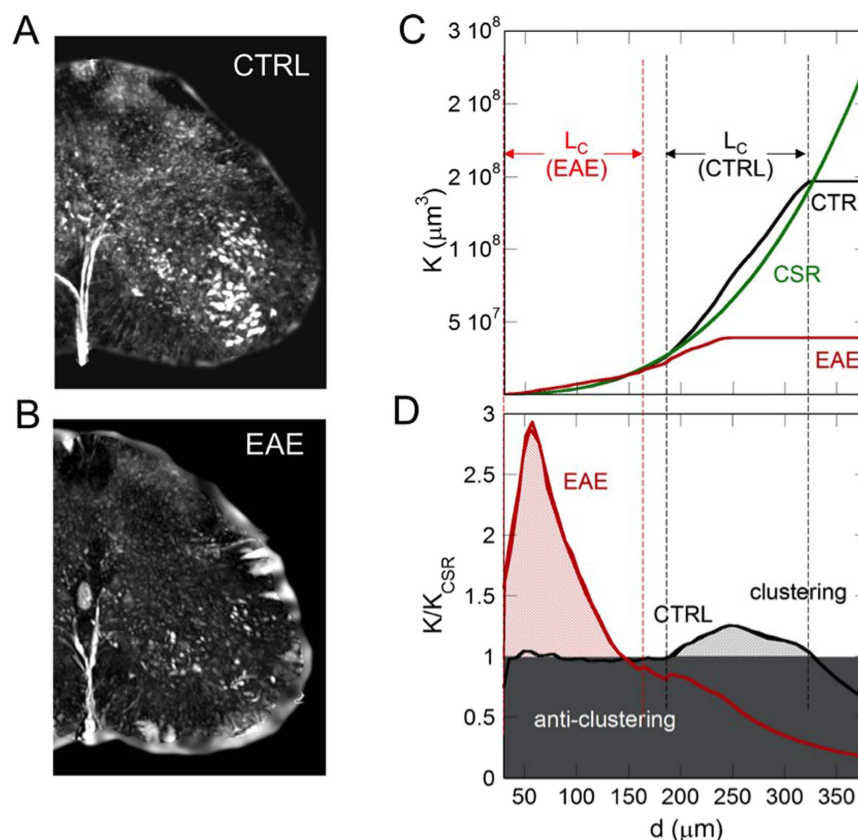
Figure 7. Phase contrast tomographic volume, 700 μm thick of (A) healthy (CTRL) and (B) EAE samples. (C) K-Ripley function of the motor neurons calculated in a typical volume of (red line) EAE and (black line) CTRL samples. The thick green lines represent the K-Ripley function of randomly located neurons. (D) K/K_{\text{CSR}} ratio, of the motor neurons calculated in the same volume of EAE (red line) and CTRL samples (black line). In the white region ( \rho > 1 ) the neurons tend to clusterize within the range lengths, L_c , indicated by the dashed lines at 145 μm and at [185–330] μm in EAE and CTRL samples, respectively.
