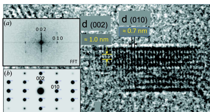
Figure 6 Main panel: HRTEM observation of a C–S–H crystal having a size of ~6 × 20 nm, formed from hydration of C 3 S in the presence of additional CaCl 2 . Vertical and horizontal solid lines, respectively, highlight the presence of periodicities of ~7 Å and, perpendicular, of 10–11 Å, which are more easily identified in the figure resulting from the fast Fourier transform of this image [inset (a)], this diagram being compatible with the calculated selected-area electron diffraction pattern [inset (b)] of tobermorite (Merlino et al. , 1999). Indexings are performed using the tobermorite (Merlino et al. , 1999) model.
