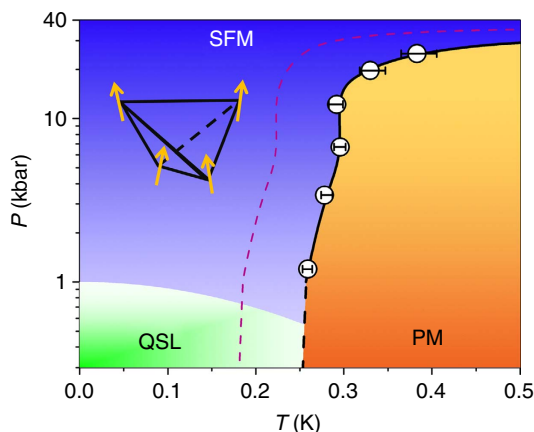
Figure 3 | Pressure-temperature phase diagram of \text{Yb}_{2+x}\text{Ti}_{2-x}\text{O}_{7+\delta} .
