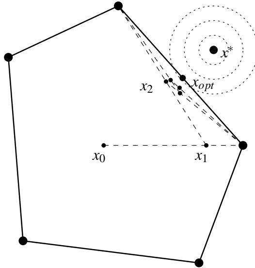
Figure 1: Zigzagging convergence of Frank and Wolfe's method
