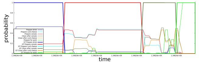
Figure 1: Probabilities of activity recognition for the morning routine from one of the 14 days in the real-world data set.
