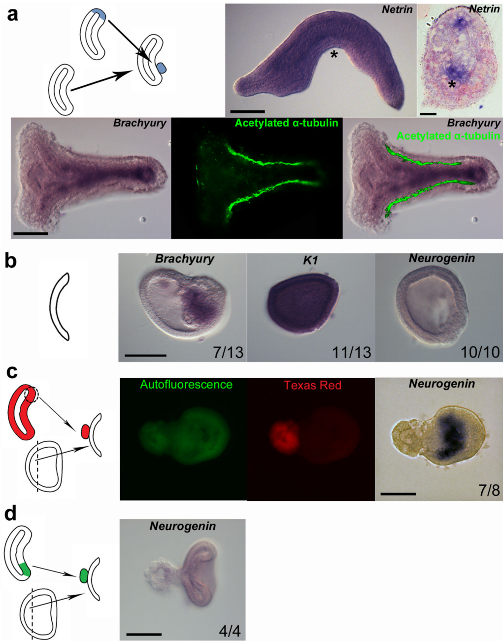
Figure 1. The dorsal blastoporal lip of amphioxus is homologous to the vertebrate organizer. a. Graft experiments were undertaken by dissecting and inserting the blastopore lip of a G2 gastrula stage embryo in the ventral archenteron of a host embryo at the same developmental stage. Some embryos showed partial double axis as indicated using the neural marker Netrin . Other embryos formed a complete double axis as indicated by expression of the notochordal marker Brachyury and by immunostaining of axons for acetylated \alpha -tubulin. The arrowhead indicates the position of the transverse section and the asterisks the ectopic expression of Netrin . b. Ectodermal explants were obtained through micro-dissection of the
