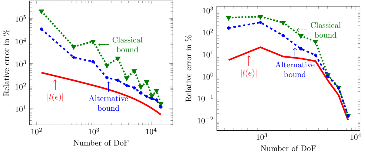
(a) Convection-dominated diffusion problem with a discontinuous diffusion coefficient ( \alpha = 10^{-4} \cdot \mathbb{1}_{(0,1) \times (0,0.5)} + 10^{-7} \cdot \mathbb{1}_{(0,1) \times (0.5,1)} ). (b) Helmholtz problem with discontinuous materials ( \gamma = 2842 \cdot \mathbb{1}_{(0,1) \times (0,0.5)} + 5053 \cdot \mathbb{1}_{(0,1) \times (0.5,1)} ).
