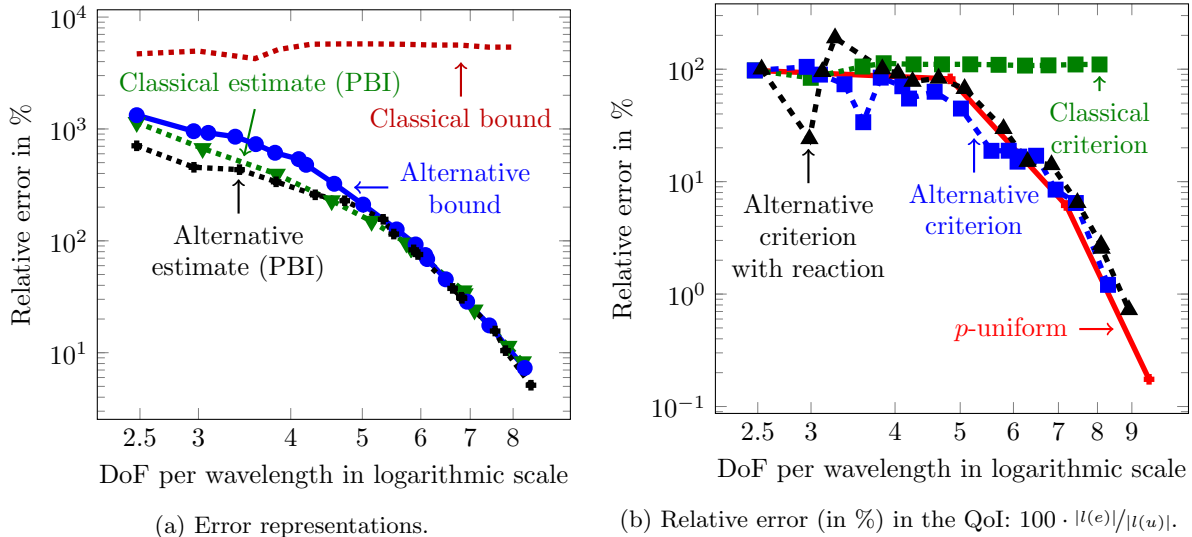
Figure 8: 2D case, k = 17\pi , hk \gg 1 . Panel (a): error representation for p -adaptivity depending on the criterion used: classical criterion \cdots , alternative criterion \bullet , classical one using PBI \cdots , and alternative one using PBI \cdots . Panel (b): error evolution in the QoI, |l(e)| depending on the adaptivity criterion: uniform p -refinements \rightarrow , p -adaptivity using the classical error representation \cdots , p -adaptivity using the alternative error representation based on the Laplacian ( \blacksquare ), and p -adaptivity using the alternative error representation based on the Laplace operator plus a positive reaction term with its coefficient being equal to k^2 ( \blacktriangle ).
