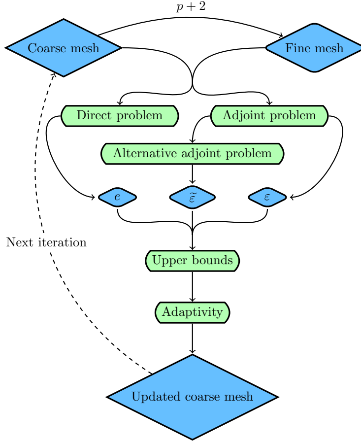
Figure 6: Algorithm of the GOA
