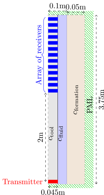
Figure 19: Sketch of the computational domain for acoustic LWD measurements, composed of three different materials: The logging tool, the borehole fluid, and the rock formation. The axis of symmetry is located on the left side of the domain, and coincides with the tool center. We have added a PML to truncate the computational domain. In red, we draw the transmitter and in blue the array of receivers.
