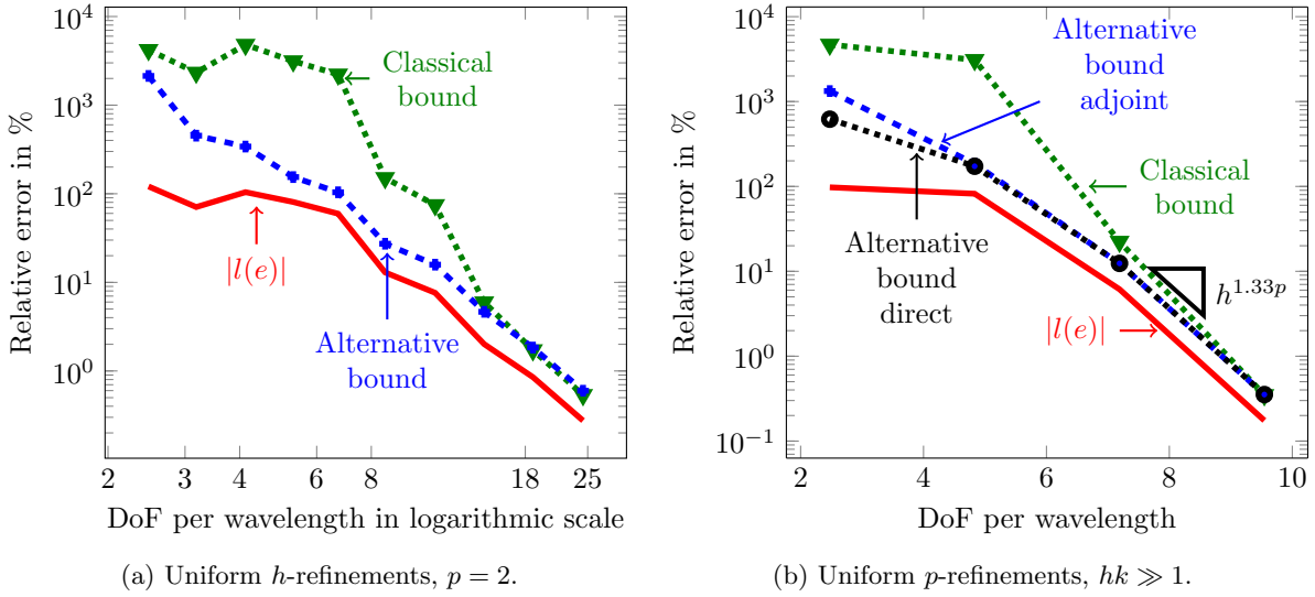
Figure 7: 2D case, k = 17\pi . Error evolution in the QoI |l(e)| (red solid line) and the upper bounds given by the different error representations, namely, the classical bound (3.5) (green dotted line with triangles), the alternative bound using the residual dual \mathcal{R}_d^h (3.7) (blue dashed line with squares), and the alternative bound using the residual primal \mathcal{R}_p^h (3.7) (black dotted line with circles).
