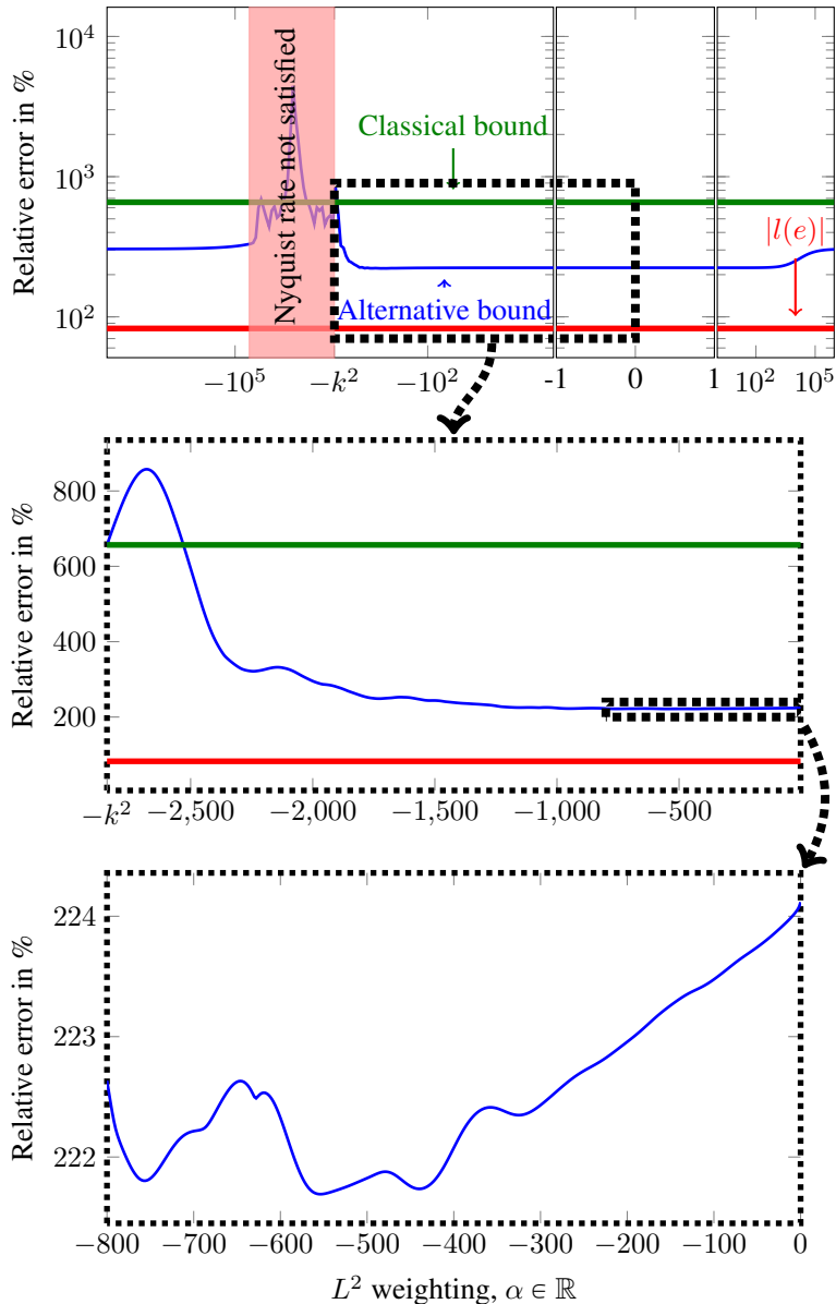
Figure 3: 2D case, \tilde{\eta}_{\mathcal{T}} versus \alpha for \alpha \in \mathbb{R} , k = 2\pi \times 8.5 = 17\pi \simeq 53 , and around 3 DoF per wavelength (with uniform p = 3 )
