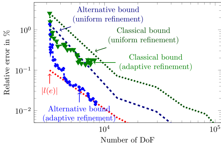
Figure 16: 2D case, convection-dominated diffusion. p -adaptivity with \nu = 10^{-7} .
