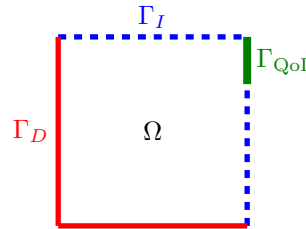
Figure 1: Computational domain in 2D
