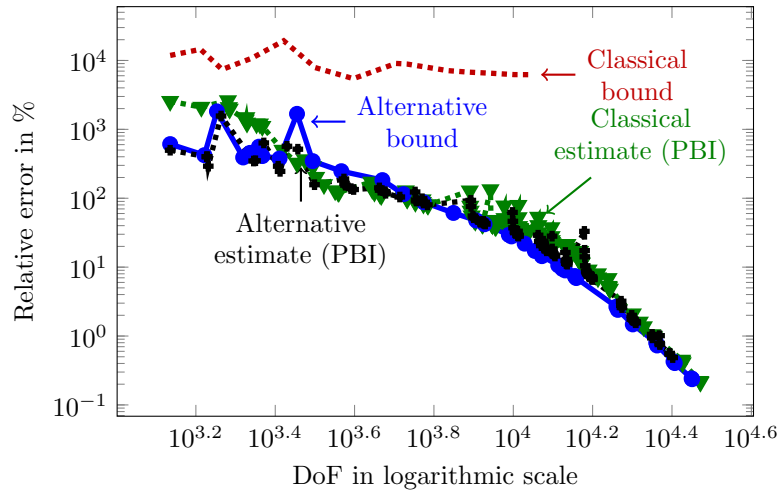
Figure 20: Sonic LWD: Error representations for p -adaptivity depending on the criterion used: classical criterion without PBI \cdots , alternative criterion without PBI \bullet , classical criterion using the PBI \blacktriangledown , and alternative criterion using the PBI \blacksquare .
