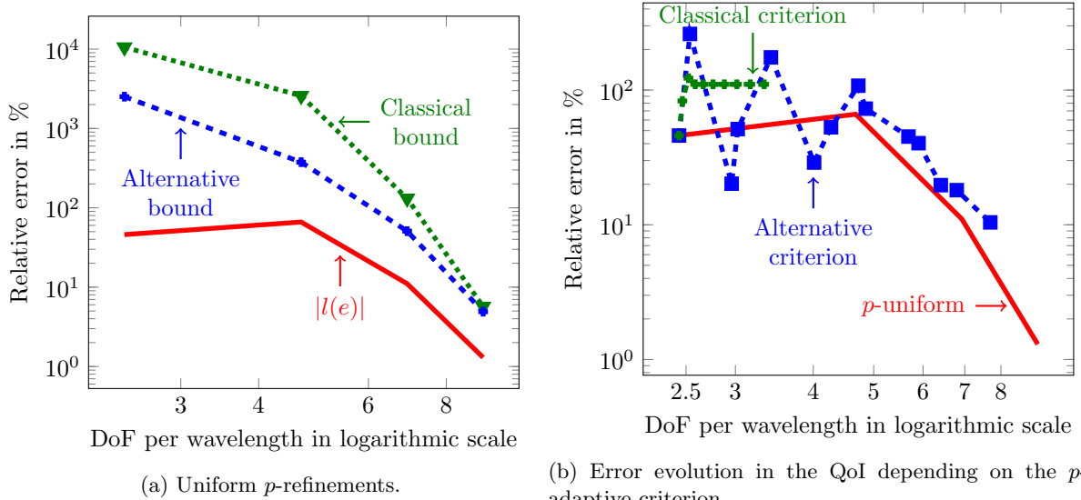
Figure 13: 3D case, k = 6\sqrt{3}\pi \simeq 32.64 .
