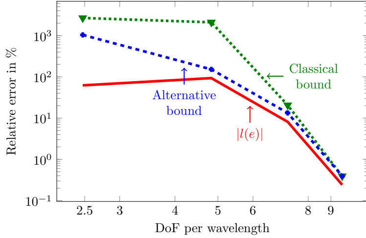
Figure 12: 2D case, k = 17\pi , hk \gg 1 , uniform p -refinements. Error evolution in the QoI and upper bounds for the error representation of the QoI when the QoI is the average of the gradient on a subdomain of \Omega .
