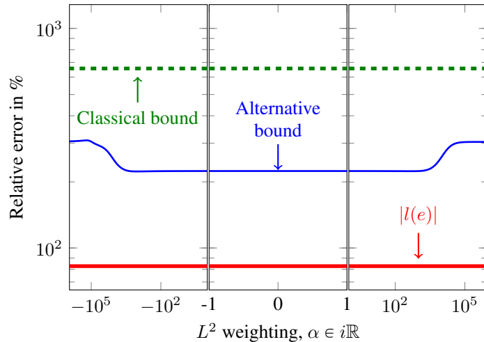
Figure 4: 2D case, \tilde{\eta}_T(\alpha) for \alpha \in i\mathbb{R} , k \simeq 17\pi , and around 3 DoF per wavelength (with uniform p = 3 )
