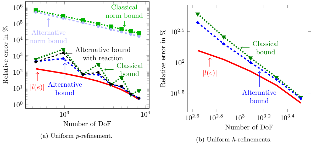
Figure 15: 2D case, convection-dominated diffusion problem. Uniform refinements for \nu = 10^{-4} .
