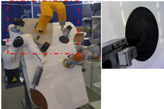
Fig. 2 Robotic solution developed for composite materials repair in the project COPERBOT
