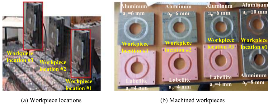
Fig. 22. Experimental results: machined workpiece.
