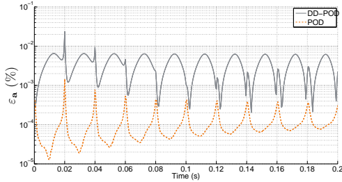
(b) Error on the solution vector for the RL load.
