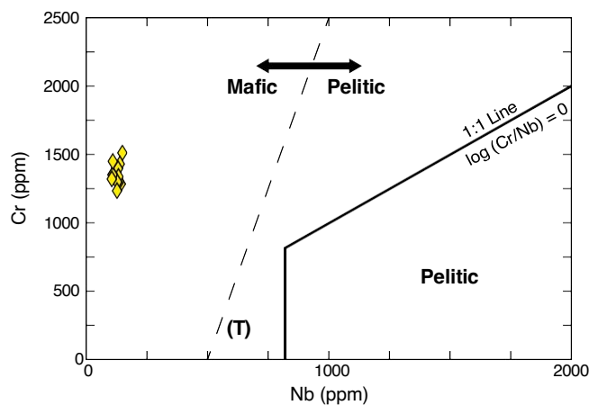
Fig. 6. Cr versus Nb diagram (Meinhold et al., 2008) for prismatic rutile from garnet megacryst ED128. The heavy dashed line is from Triebold et al. (2012) and delimits the field of metamafic and metapelitic rutile.
