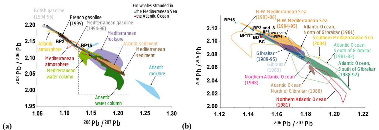
Fig. 1. 206 Pb/ 207 Pb and 208 Pb/ 206 Pb in baleen plates of fin whales stranded in the Mediterranean Sea (blue triangles) and in the Atlantic Ocean (red triangles) (a) Comparison with different Pb sources, the dashed square is the enlargement in b. (b) Comparison with data of water columns (year
