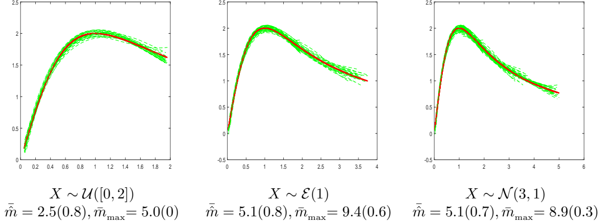
FIGURE 4. 25 estimated curves in Laguerre basis (dotted -green/grey), the true in bold (red), n = 1000 , b(x) = 4x/(1+x^2)\mathbf{1}_{x \geq 0} and different laws for the design.
