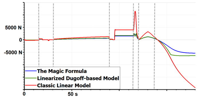
Fig. 10. AMESim ® comparison of Pacejka model with linearized models - Front left tire lateral force.
