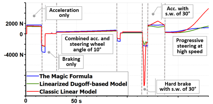
Fig. 9. AMESim ® comparison of Pacejka model with linearized models - Front left tire longitudinal force.
