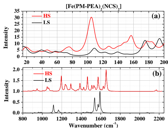
Figure 9: Computed IR (a) and Raman (b) spectrum of the [\text{Fe}(\text{PM-PEA})_2(\text{NCS})_2] complex.
