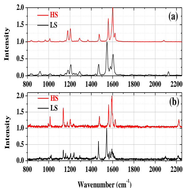
Figure 2: Raman Spectra of of (a) [\text{Fe}(\text{PM-BiA})_2(\text{NCS})_2] and (b) [\text{Fe}(\text{PM-PEA})_2(\text{NCS})_2] .
