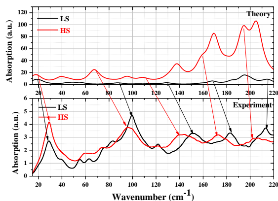
Figure 8: Comparison of the normalized experimental and computed IR spectra of the [\text{Fe}(\text{PM-BiA})_2(\text{NCS})_2] complex.
