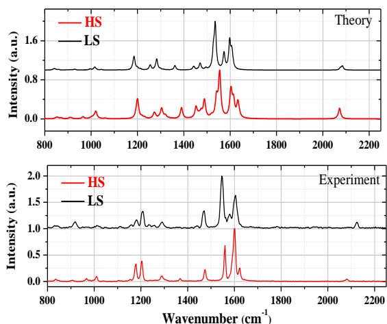
Figure 6 : Comparison of the normalized experimental and computed Raman spectra of the [\text{Fe}(\text{PM-BiA})_2(\text{NCS})_2] complex.
