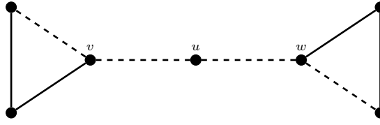
Figure 3: A decomposition into two nice bipartite graphs mentioned in the proof of Lemma 5.8. Solid edges stand for red edges. Dashed edges stand for blue edges.
