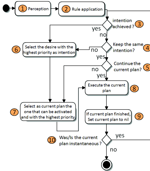
Figure 1. Activity diagram
