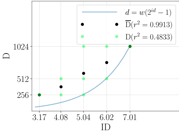
Figure 2. The 9 \mathcal{D} conditions (light green dots) that lead to the 5 ID conditions used in the thought experiment. Black dots correspond to \bar{D} , the average value of D for equal IDs. Dark green dots correspond to data points that overlap the average. r^2 between D and ID and between \bar{D} and ID are given in the legend. The blue line corresponds to Eq. 8.
