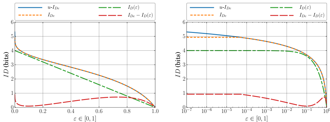
Fig. 8. Comparison of ID(\epsilon) and ID_e for erasure rate in [0, 1] , for \frac{D}{W} = 15 . u-ID_e refers to ID_e where the 0.0049% distinction is not made. The scale is lin-lin left and lin-log right.
