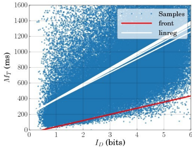
Fig. 10. Same data as in Figure 9, with the Y-axis cut at 1.6 s. Shown are linear fits from usual linear regression ('linreg' in white), using a number of different thresholds for the exclusion of outliers, as well as an estimation of the front of performance (in red).
