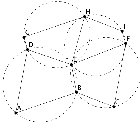
Figure 1: Illustration of the notation for a biperiodic circle pattern with both periods equal to two.
