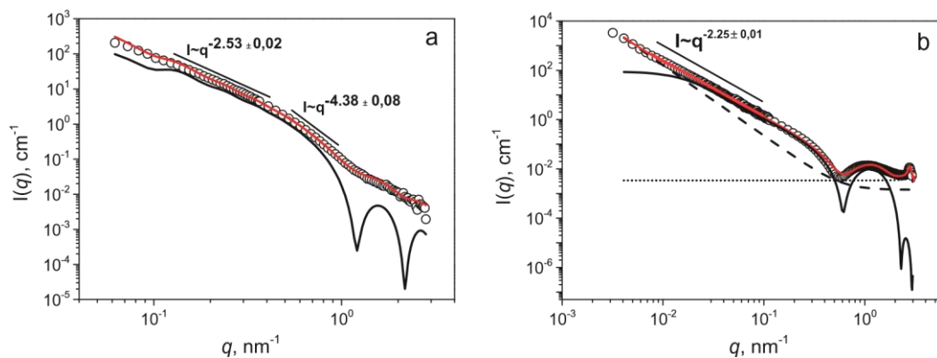
Fig. 3. SANS (a) and SAXS (b) curves of PMeOx_{30} -b- POctOx_{20} solutions prepared by direct dissolution. Symbols are experimental scattering data, and red solid lines are fits generated as described in the text. The black solid lines are the form factors of bilayered vesicles, the black dashed lines are the form factors of large aggregates and the black short dotted lines describe the Voigt peak contribution. (For interpretation of the references to colour in this figure legend, the reader is referred to the web version of this article.)
