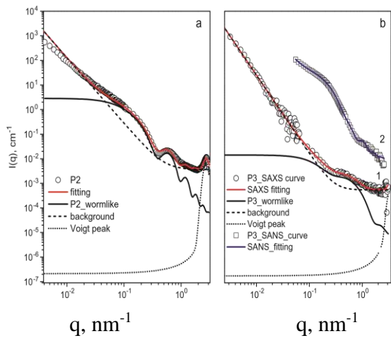
Fig. 6. SAXS (a and b) and SANS (curve no 2 in Fig. 5b) data for PMEO 33 -b-POctOx 23 -C 16 F 21 (P2) and PMEO 33 -b-POctOx 23 -C 12 F 21 (P3) solutions prepared by direct dissolution. Symbols are experimental scattering data. Solid lines are fits generated as described in the text. The black solid lines are form factors of wormlike micelles; black short dashed lines are the form factors of large aggregates and the black short dotted lines are the Voigt peak contributions.
