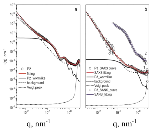
Fig. 6. SAXS (a and b) and SANS (curve no 2 in Fig. 5b) data for \text{PMeOx}_{33}\text{-b-POctOx}_{23}\text{-C}_{16}\text{F}_{21} (P2) and \text{PMeOx}_{33}\text{-b-POctOx}_{23}\text{-C}_{12}\text{F}_{21} (P3) solutions prepared by direct dissolution. Symbols are experimental scattering data. Solid lines are fits generated as described in the text. The black solid lines are form factors of wormlike micelles; black short dashed lines are the form factors of large aggregates and the black short dotted lines are the Voigt peak contributions.
