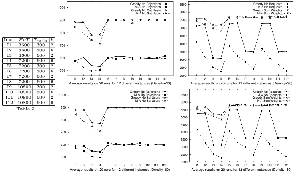
Fig. 5: Comparison between the Greedy model and the Multi-Agent one using different values of k , T_{min} , EoT and density
