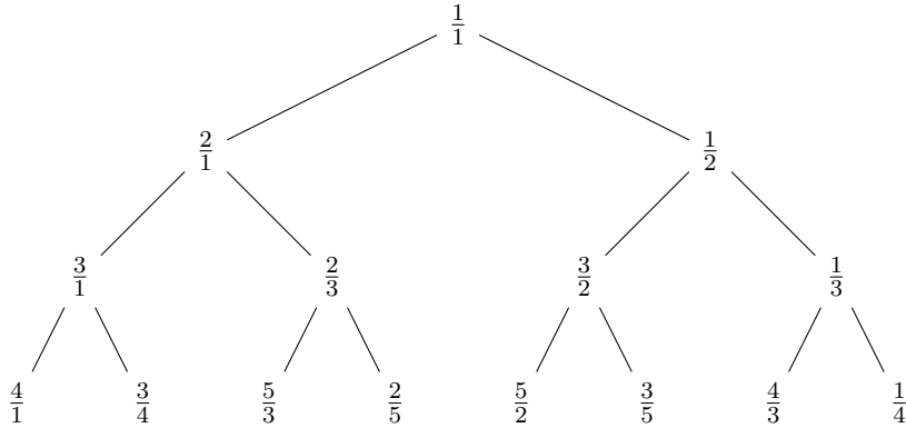
FIGURE 2. First four rows of the Calkin-Wilf tree
