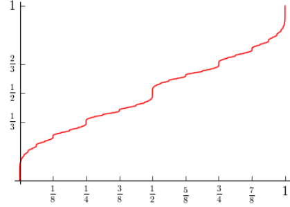
FIGURE 3B. Graph of Conway's box function \Phi(x) = ?^{-1}(x) .
