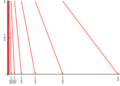
FIGURE 4B. Graph of the jump transformation x \mapsto \mathcal{B}_\triangleright(x) .
