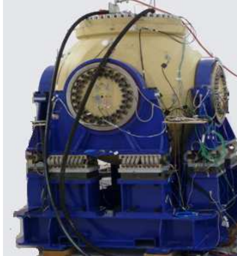
Figure 2: Picture of the studied containment vessel
