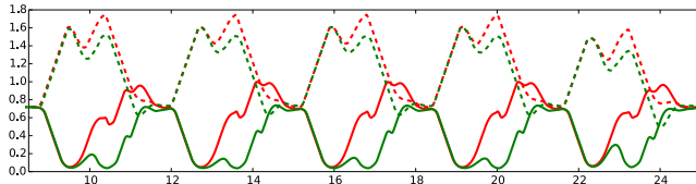
Fig. 8. Knee angle variations between LIP-based (red) and VHIP-based (green) whole-body control. Solid lines correspond to the right knee and dashed ones to the left knee. The right knee stays extended longer in the VHIP pattern, curtailing a peak in left-knee flexion observed in the LIP pattern.
