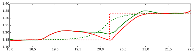
Fig. 7. CoM height variations for LIP-based (red) and VHIP-based (green) walking patterns on a representative step. Dashed lines: references from walking patterns. Solid lines: estimates by the controller's CoM observer. Tracking cannot be perfect as walking patterns do not take into account swing foot motions (18.5–20.0 s) and maximum leg extension during double support (20.0–20.2 s) that limit the CoM height kinematically.
