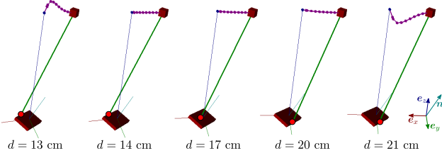
Fig. 3. Zero-step capture trajectories for different contact locations. The horizontal distance d from CoM to contact varies while the initial CoM position and velocity are kept constant. Red discs indicate the instantaneous CoP location r_i . The regularization cost keeps the trajectory as close as possible to a LIP via CoP variations. When there is no linear solution, height variations are resorted to for additional acceleration or braking.
