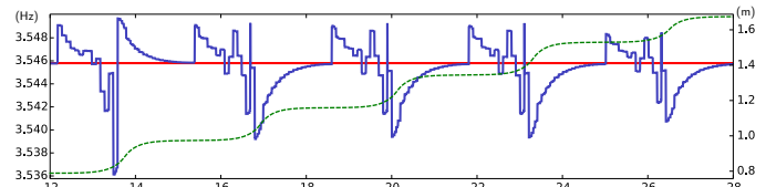
Fig. 10. Time-varying frequency \omega(t) of the VHIP (blue) compared to its LIP counterpart (red). The VHIP pattern CoM height (Figure 7) is shown for reference in green. The frequency rises when the DCM accelerates upward and falls when the DCM accelerates downward.
