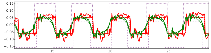
Fig. 9. Lateral DCM-ZMP tracking for the VHIP over the complete stair climbing motion. Green: DCM, red: ZMP, dashed: reference, solid: observed. The DCM here is the position \mathbf{c}(t) + \dot{\mathbf{c}}(t)/\omega(t) . References look like a regular capture-point pattern generator as the variations of \omega(t) required to lift the robot up by 18.5 cm are too small to affect the robot's lateral dynamics. The same behavior is observed on sagittal dynamics.
