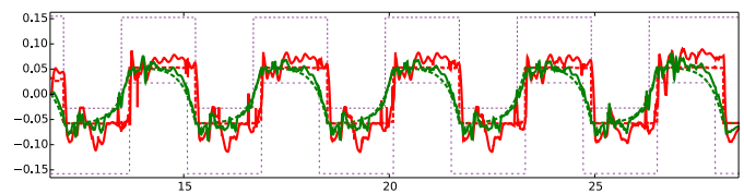
Fig. 9. Lateral DCM-ZMP tracking for the VHIP over the complete stair climbing motion. Green: DCM, red: ZMP, dashed: reference, solid: observed. The DCM here is the position c(t) + \dot{c}(t)/\omega(t) . References look like a regular capture-point pattern generator as the variations of \omega(t) required to lift the robot up by 18.5 cm are too small to affect the robot's lateral dynamics. The same behavior is observed on sagittal dynamics.
