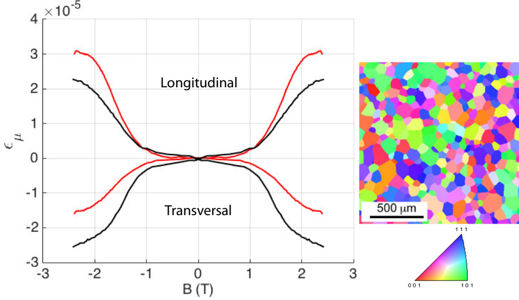
FIG. 6. Magnetostrictive behavior of Fe-27%Co with crystallographic map associated (IPF - ND) for a sample annealed in ferritic phase and fast cooling (red curve along RD, black curve along TD).
