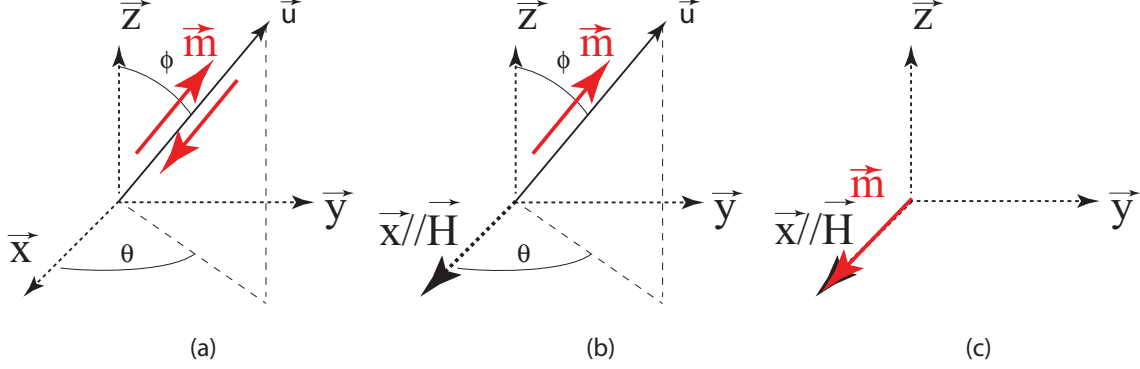
FIG. 4. Ideal magnetization process of samples annealed in the ferritic domain.
