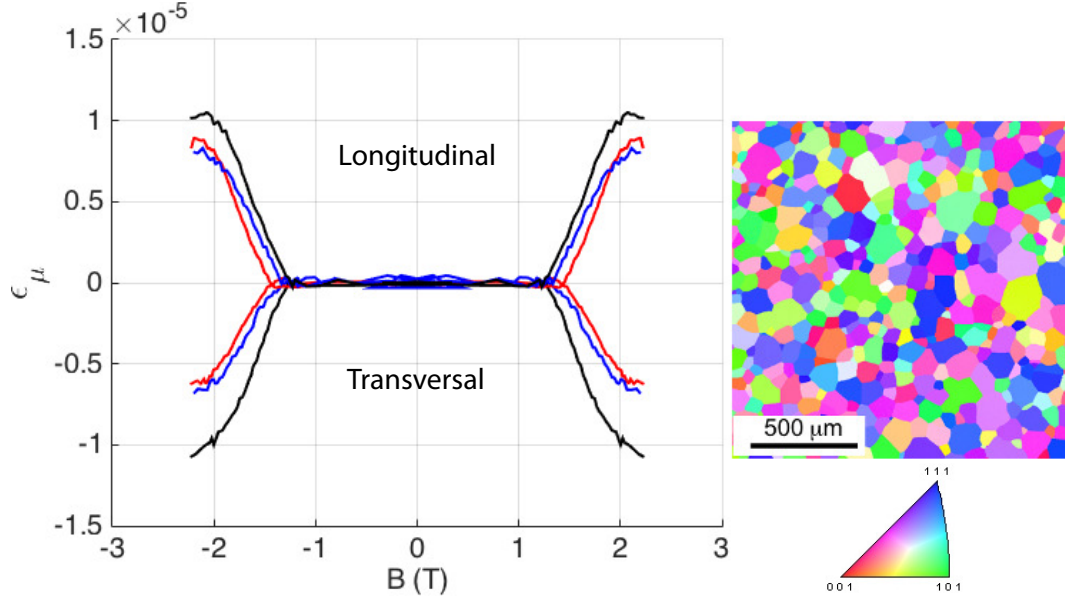
FIG. 1. Magnetostrictive behavior of Fe-27%Co with crystallographic map associated (IPF - ND) for a sample annealed in ferritic phase (red curve along RD, blue curve along 45°/RD, black curve along TD).
