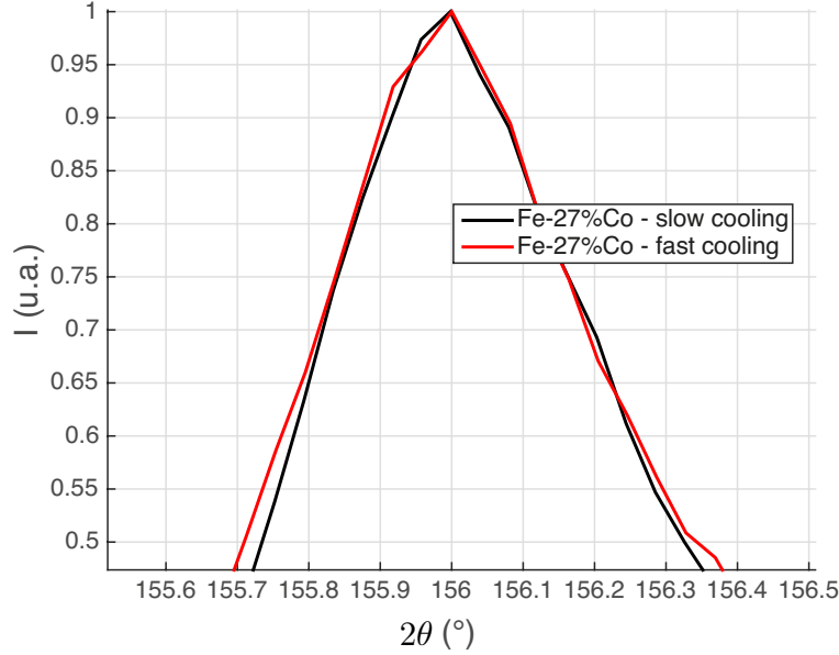
FIG. 7. Compared position of X-Ray diffraction peaks of \{211\} planes for fast (red curve) or slow (black curve) cooling after final annealing at T_3=900^\circ\text{C} -1h-pure H 2 .
