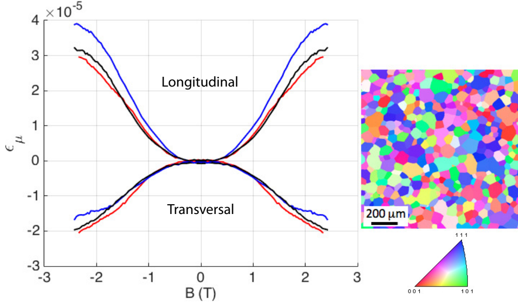
FIG. 2. Magnetostrictive behavior of Fe-27%Co with crystallographic map associated (IPF - ND) for a sample annealed in austenitic phase (red curve along RD, blue curve along 45°/RD, black curve along TD).
