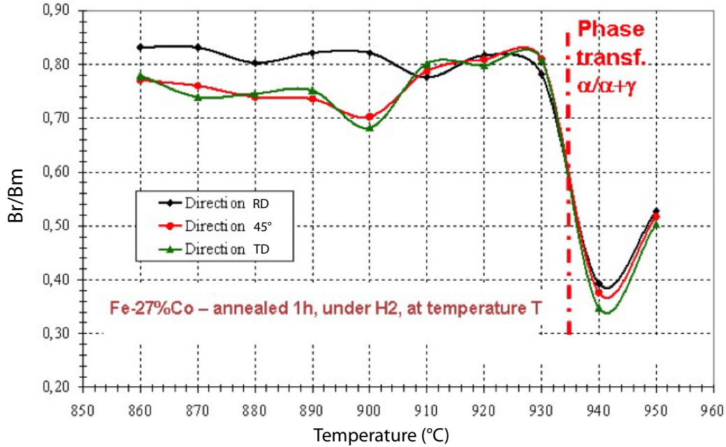
FIG. 5. Reduced remanent induction Br/B_m versus annealing temperature.
