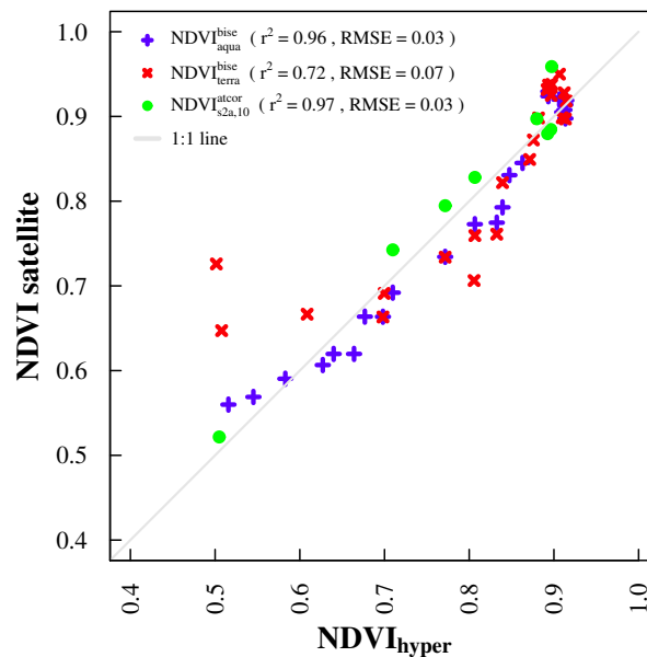
Figure 7. Scatter-plot of NDVI derived from the hyperspectral sensor system ( NDVI_{hyper} ) and satellite NDVI products ( NDVI_{satellite} ). Satellite NDVI products include NDVI_{aqua}^{bise} (blue), NDVI_{terra}^{bise} (red), as well as NDVI_{s2a,10}^{atcor} (green). NDVI_{multi} and NDVI_{s2a,20}^{atcor} are not shown due to large similarities with NDVI_{hyper} and NDVI_{s2a,10}^{atcor} , respectively.
