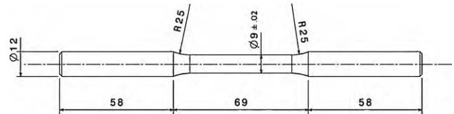
Fig. 2. Fatigue specimen geometry (dimensions in mm).
