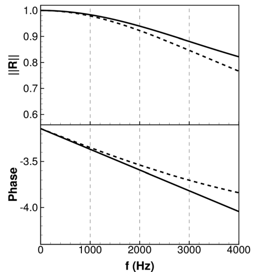
Fig. 3 Modulus and phase of the reflection coefficient R of the combustion chamber outlet: — Levine and Schwinger [31], - - - AVBP with adequate relaxation coefficient
