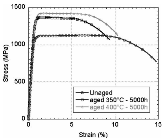
Fig. 5 Stress–strain curves for 15-5 PH, unaged and aged 5000 h at 350 and 400 °C
