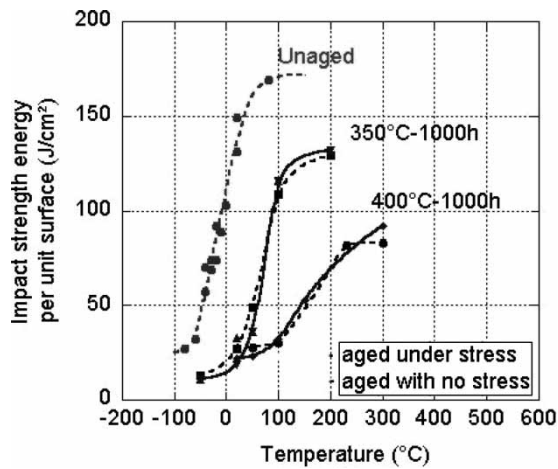
Fig. 9 Ductile to brittle transition for alloy 15-5 PH, unaged and aged under stress 1000 h at 350 and 400 °C
