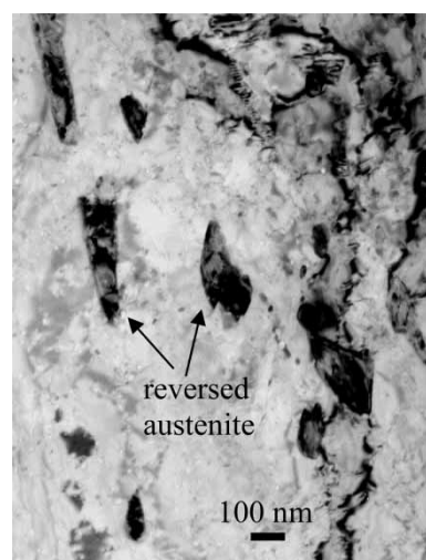
Fig. 2 TEM micrograph showing reversed austenite
