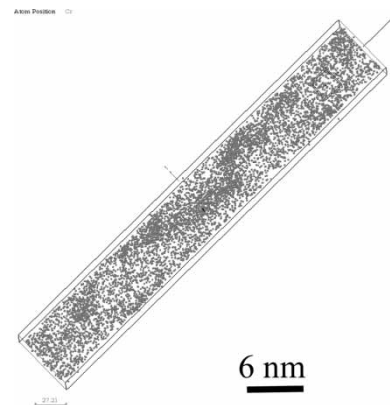
Fig. 7 Distribution of Cr atoms in alloy aged 1000 h at 400 °C (atomic probe)
