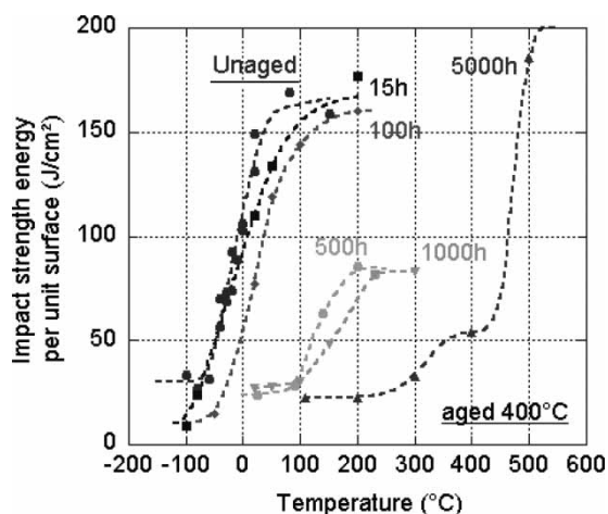
Fig. 4 Ductile to brittle transition for alloy 15-5 PH, unaged and aged at 400 °C
