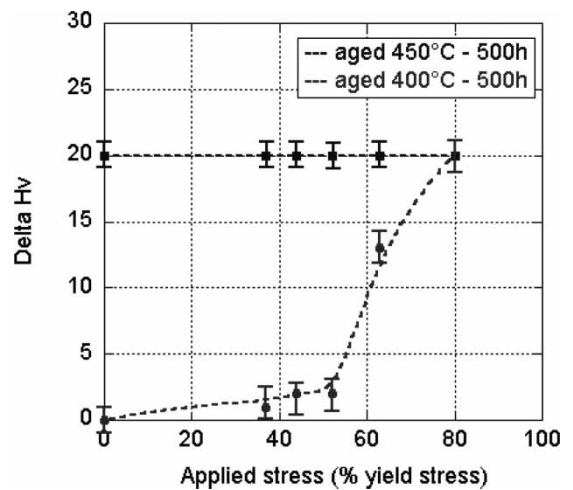
Fig. 10 Difference \Delta H_v in Vickers hardness between unaged alloy and alloy aged under stress at 400 and 450 °C
