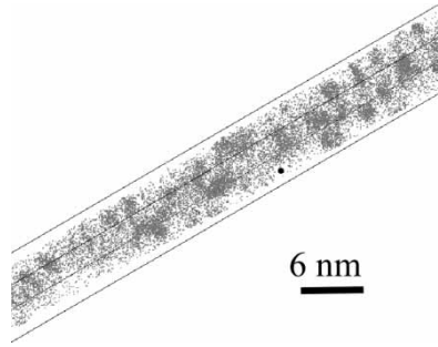
Fig. 8 Distribution of Cr atoms in alloy aged 5000 h at 400 °C (atomic probe)
