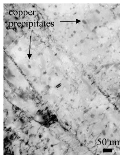
Fig. 1 TEM micrograph showing the fine precipitation of copper particles
