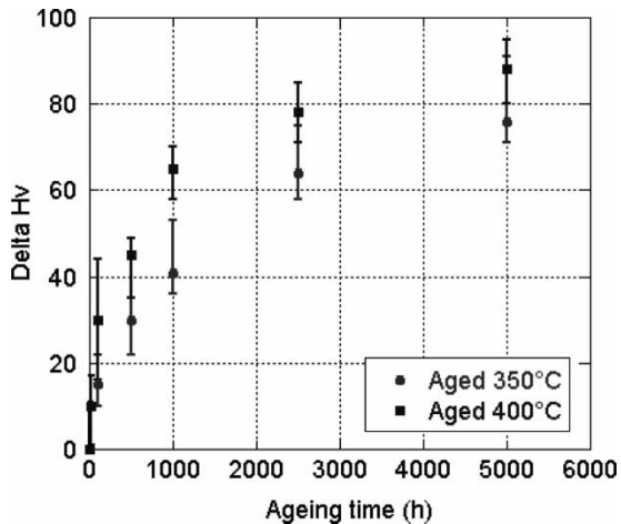
Fig. 6 Difference \Delta H_v in Vickers hardness between unaged alloy and alloy aged at 350 and 400 °C
