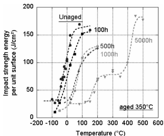
Fig. 3 Ductile to brittle transition for alloy 15-5 PH, unaged and aged at 350 °C
