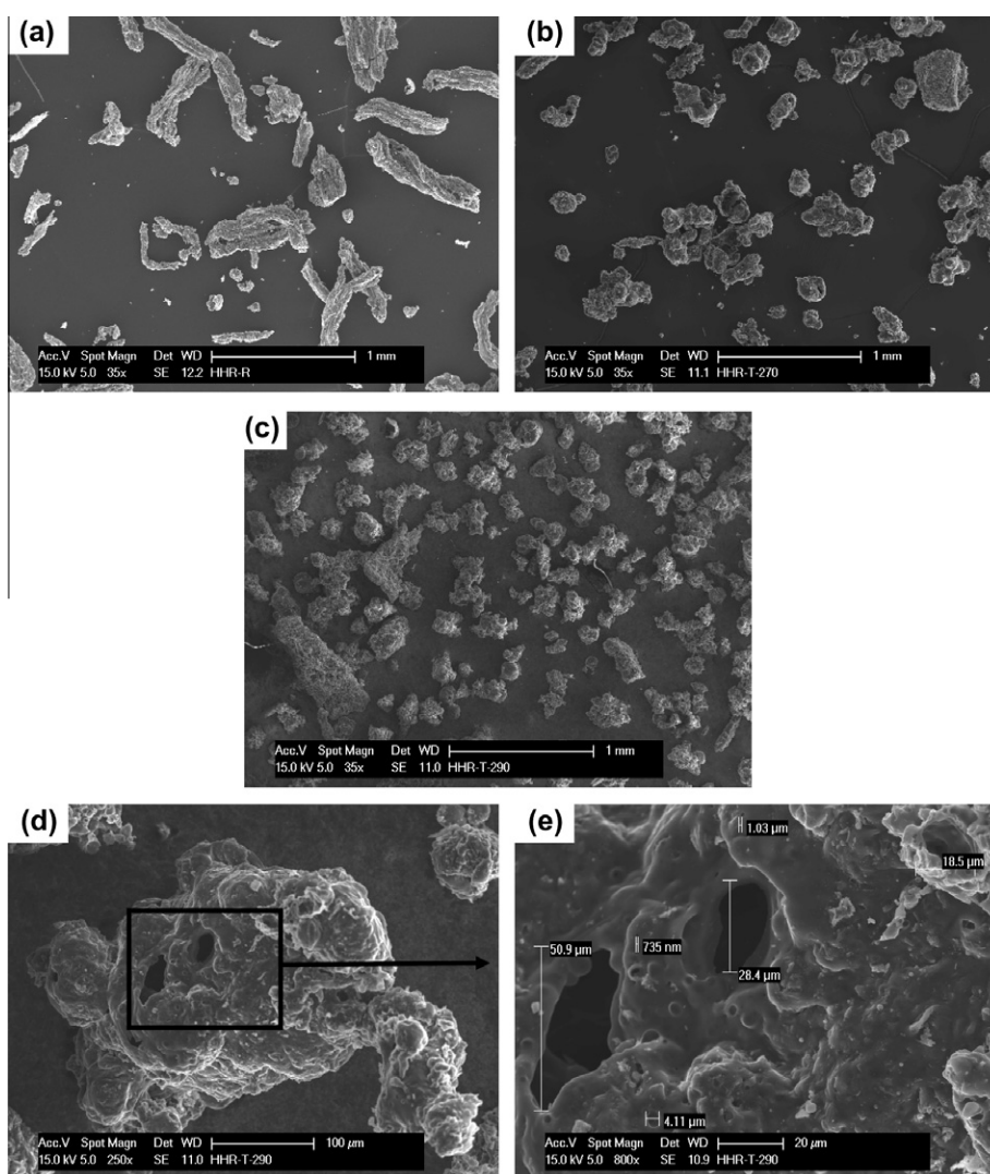
Fig. 4. SEM images of chars: (a) HHR-R; (b) HHR-T-270; (c-e) HHR-T-290; image (e) is a zoom of the rectangular zone shown in image (d).
