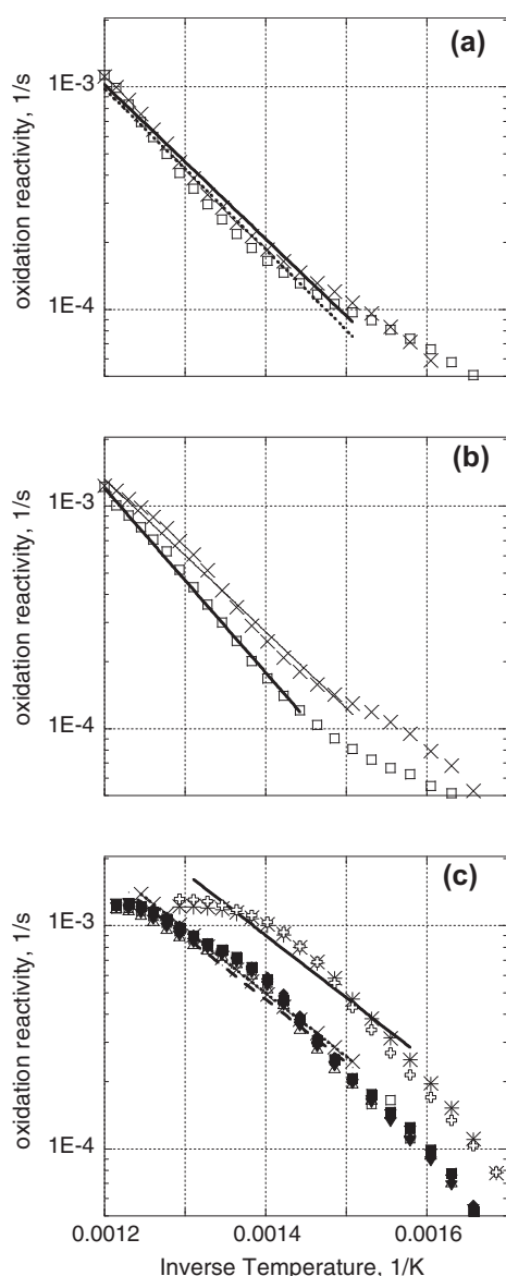
Fig. 5. Oxidative reactivity Arrhenius plots. Lines show the range over which the Arrhenius fits of Table 4 were obtained. (a) chars produced at low heating rates to 1000 °C. exes: char from raw biomass (LHR-1000-R); squares: char from torrefied biomass (LHR-1000-T-290). (b) chars produced at low heating rates to 850 °C. exes: char from raw biomass (LHR-850-R); squares: char from torrefied biomass (LHR-850-T-290). (c) chars produced at high heating rates. Crosses and exes: char from raw biomass (HHR-R); triangles: char from biomass torrefied to 270 °C (HHR-T-270); squares: char from biomass torrefied to 290 °C (HHR-T-290).
