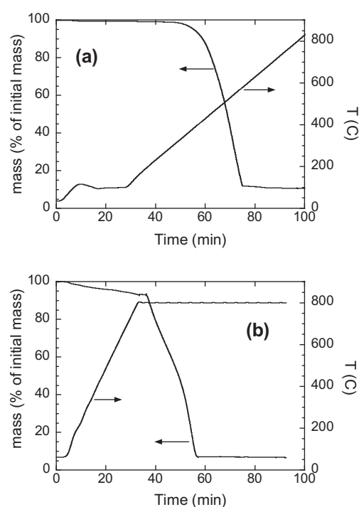
Fig. 1. Representative TGA mass and temperature profiles, for char HHR-T-290, for (a) oxidation; (b) gasification.
