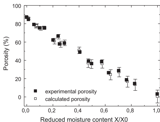
Fig. 18 – Experimental and calculated porosity of potato as a function of the water content: freeze drying (Krokida and Maroulis, 1997).
