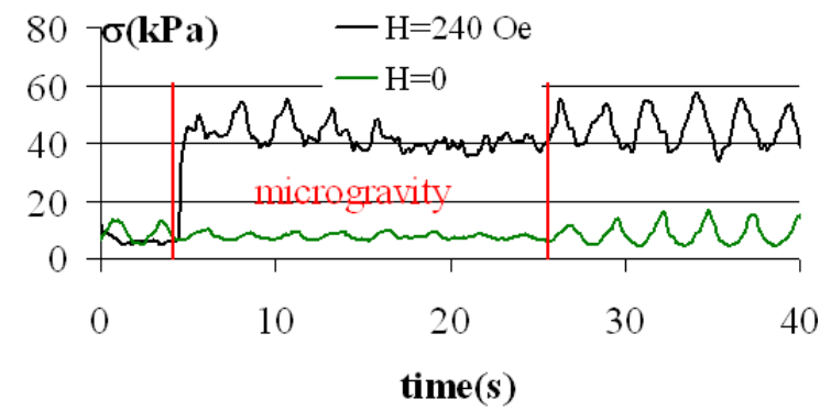
Figure 8. Stress versus time at a constant shear rate of 11\text{ s}^{-1} with the vane geometry in microgravity experiments upper curve: H=240 Oe; lower curve H=0 .
