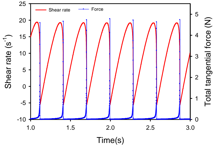
Fig19 In red the shear rate calculated for a viscoelastic liquid through Eqs (16)-(14) for a constant applied stress: \sigma_a=50\text{Pa} ; the shear modulus is given by Eq.(15) with G_0=3\text{Pa} and the parameter for the second viscosity was \alpha=2 . In blue the total tangential force corresponds to the right axis.
