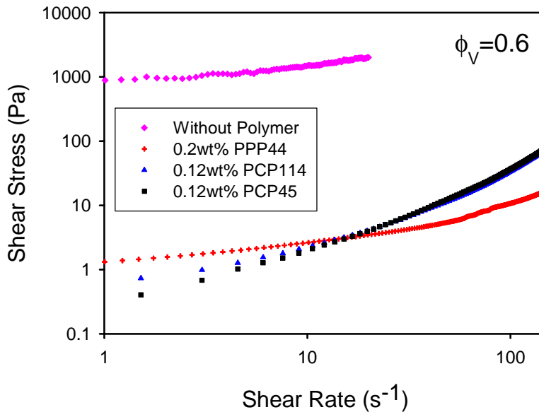
Fig.4 Comparison of the rheograms- shear stress versus shear rate- of a suspension of calcium carbonate at volume fraction \Phi=60\% without dispersant (upper curve) and with each of the three polymers
