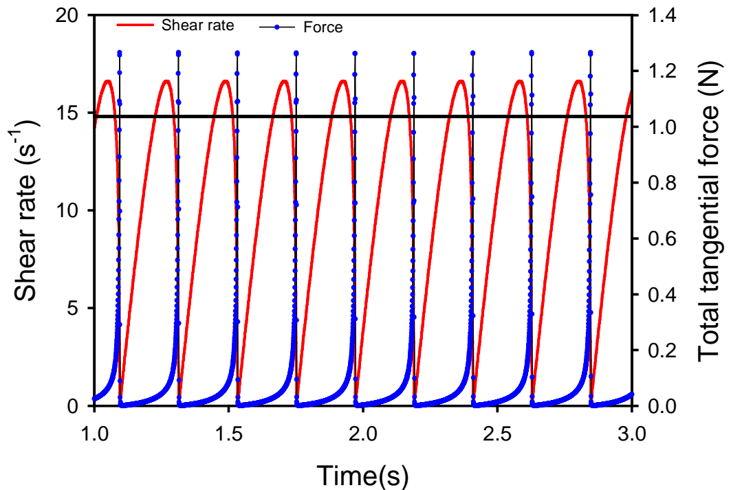
Fig 18 Shear rate calculated from Eqs (11)-(14) for a constant applied stress: \sigma_a = 50Pa ; in black using f(\sigma_a) for the fraction of frictional contacts and in red f(\sigma_s) where \sigma_s is the total stress including the inertial one (cf. Eq.(11)). The blue curve represents the total tangential force. The force of 1.26N corresponds to a shear stress \sigma_s = 1000Pa
