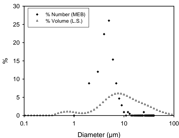
Fig.2 Size distribution obtained by counting the particles above 1μm from MEB pictures and from light scattering (L.S.) with Mastersizer 2000 from Malvern
