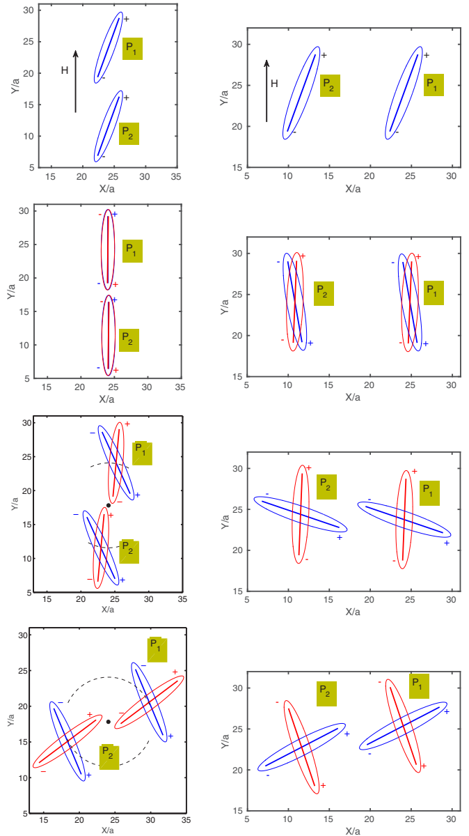
FIG. 2. Effect of the frequency on the behavior of two fibers under alternating magnetic field in the absence of HI. Left (case A) and right (case B) columns correspond to different initial configurations with the line joining fiber centers aligned with (and, respectively, perpendicular to) the magnetic field direction. The + and - charges are placed at the extremity of the continuous lines following the ellipsoid major axis. The magnetic moment of every particle is oriented from - to +. The first row corresponds to the initial state of the system. The second to fourth rows correspond to dimensionless frequencies f\tau_r = 0.023, 0.069 , and 0.138 , respectively, with HM = 10^{10} and H/M = 1 . In these rows, blue and red colors correspond to the system configuration at chosen time t and t + 1/(2f) , respectively. The circular arcs indicate the relative trajectory of the center of P_2 with respect to P_1 in time.
