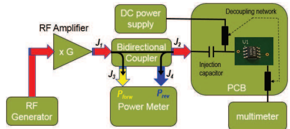
Fig. 4. Illustration of the DPI setup
