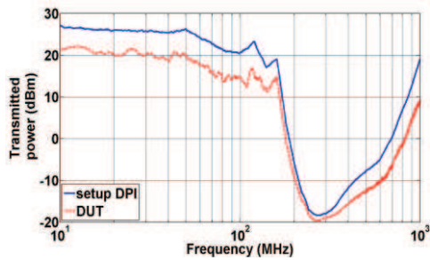
Fig. 6. Transmitted power (dBm) – V_{dd} pin
