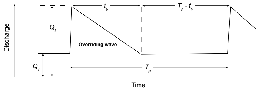
Figure 7: Schematic longitudinal elevation profile (a, modified after Thompson, 1968 ) and discharge time series (b) of a pulsated flow showing all useful variables for time-averaged discharge estimation. A more realistic profile of the roll waves is plotted in light gray (a, according to Brock's experiments reported by Richard and Gavriluk, 2012 ). D_1 , V_1 , Q_1 , are the depth, velocity, discharge, respectively, of the base flow. L_w , h_w , V_w , Q_w , are the length, height, mean velocity, mean discharge, respectively, of the surge. T_p is the time period between pulses, and t_b the transit time of pulse waves. The total flow depth at surge fronts, D_2 , is equal to D_1 + h_w . The total discharge at surge fronts, Q_2 , is considered over the full flow depth.
