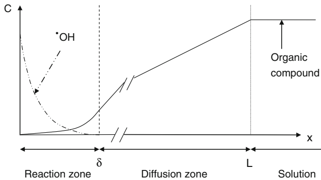
Fig. 2 Schematic representation of concentration profiles of hydroxyl radicals and of an organic compound using the BDD anode
