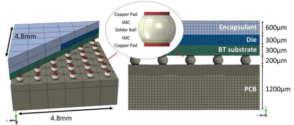
Fig. 5 : Geometry of a quarter BGA
