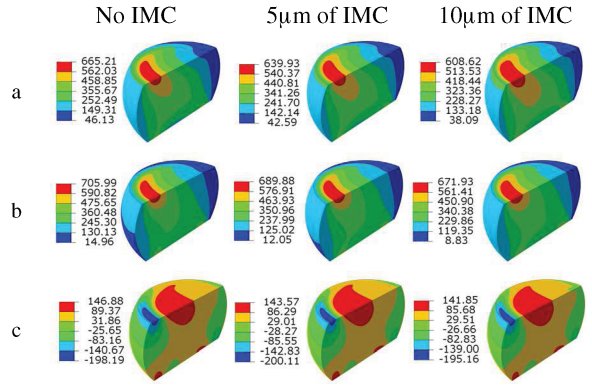
Fig. 13 : Stress distribution (MPa) in NSMD balls (a) von Mises stress ; (b) normal tensile stress ; (c) shear stress
