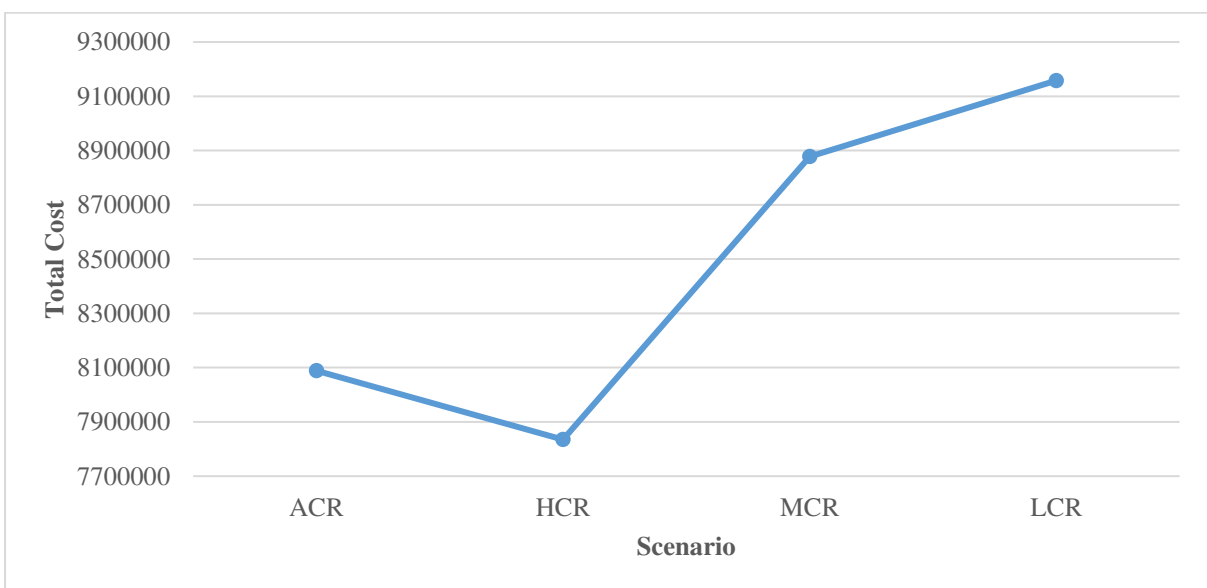
Fig. 11. The total cost vs various scenarios of capacitated rakes
