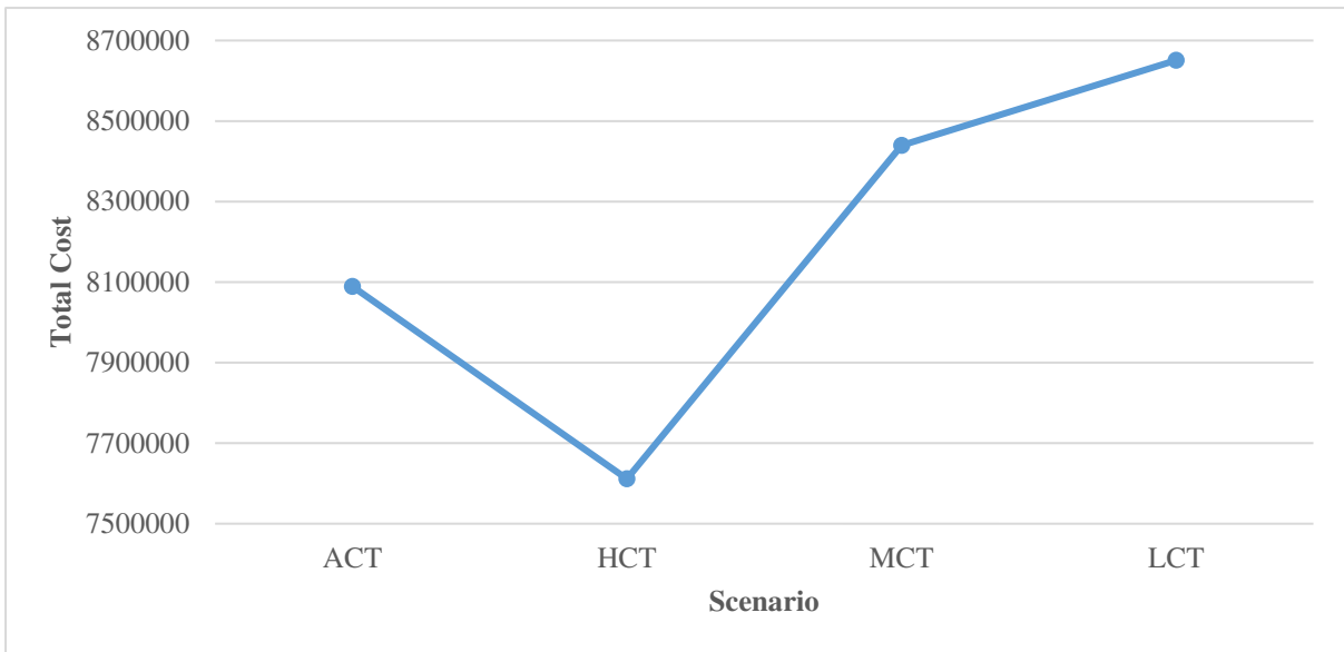
Fig. 10. The total cost against various scenarios of capacitated trucks
