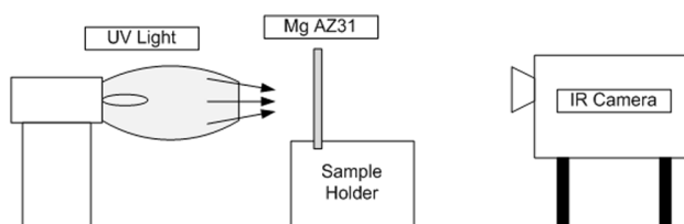
Figure 1. Selective annealing experimental setup.
