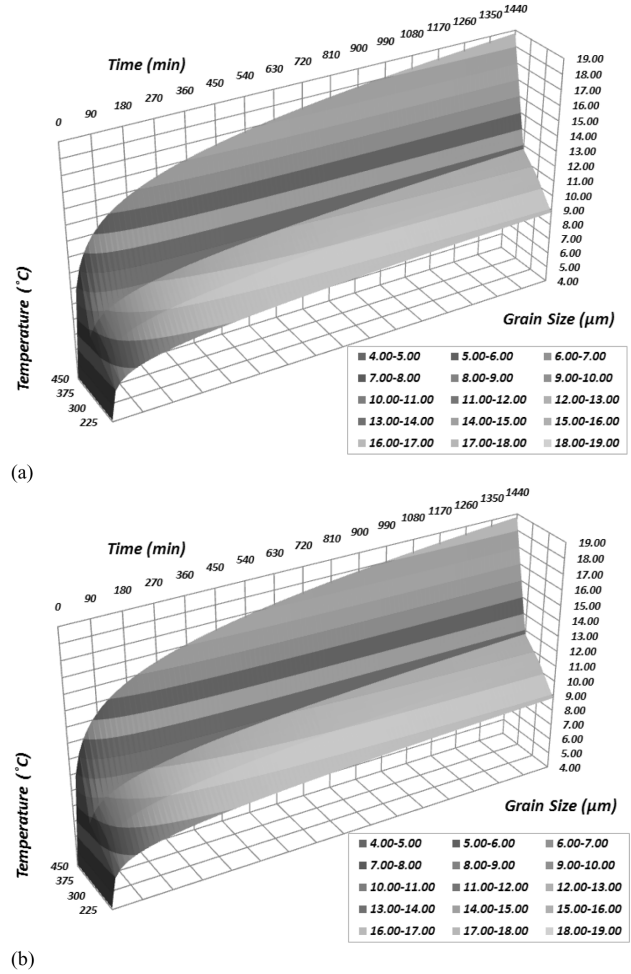
Figure 3. Static grain growth contour plots for the AZ31 magnesium alloy (a) 3.22 mm thick sheets (b) 1.07 mm thick sheets.
