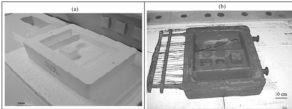
Figure 1. a: Silica based ceramic die; b: cast steel die.
