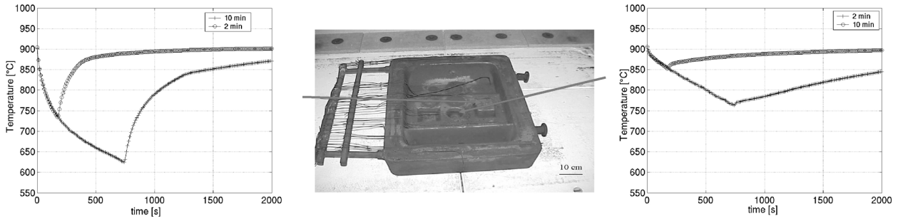
Figure 3. Thermal cycles at different locations at the surface of the tool for several cooling times.
