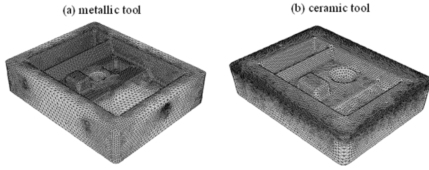
Figure 5. Finite Element meshes of the metallic (a) and ceramic (b) tools.
