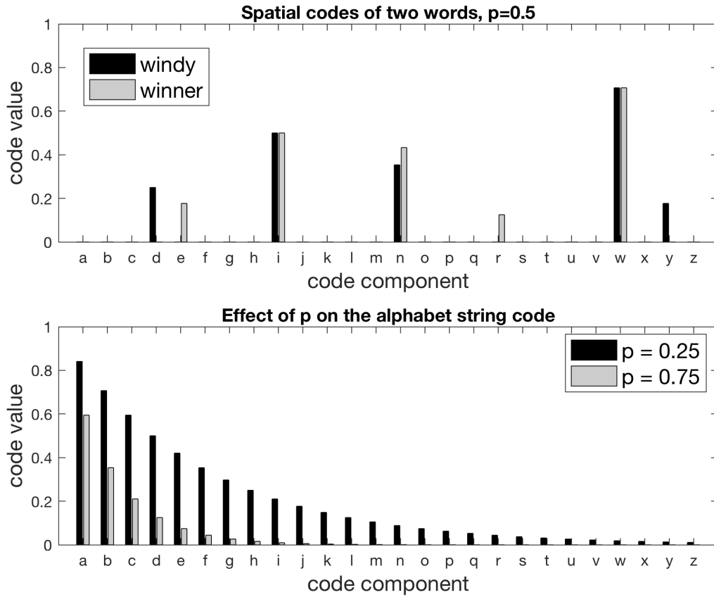
Figure 1. Visualization of the numerical spatial codes of two words (windy, winner), and of the effect of the parameter p ( p = 0.25 , or p = 0.75 ) on the alphabet string code (abcdefghijklmnopqrstuvwxyz).
